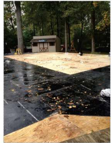
Bil-Jax staging setup and leveled to match up flush with the I beams
