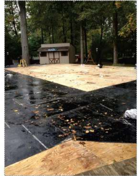
Bi-Jax staging setup and leveled to match up flush with the I beams
